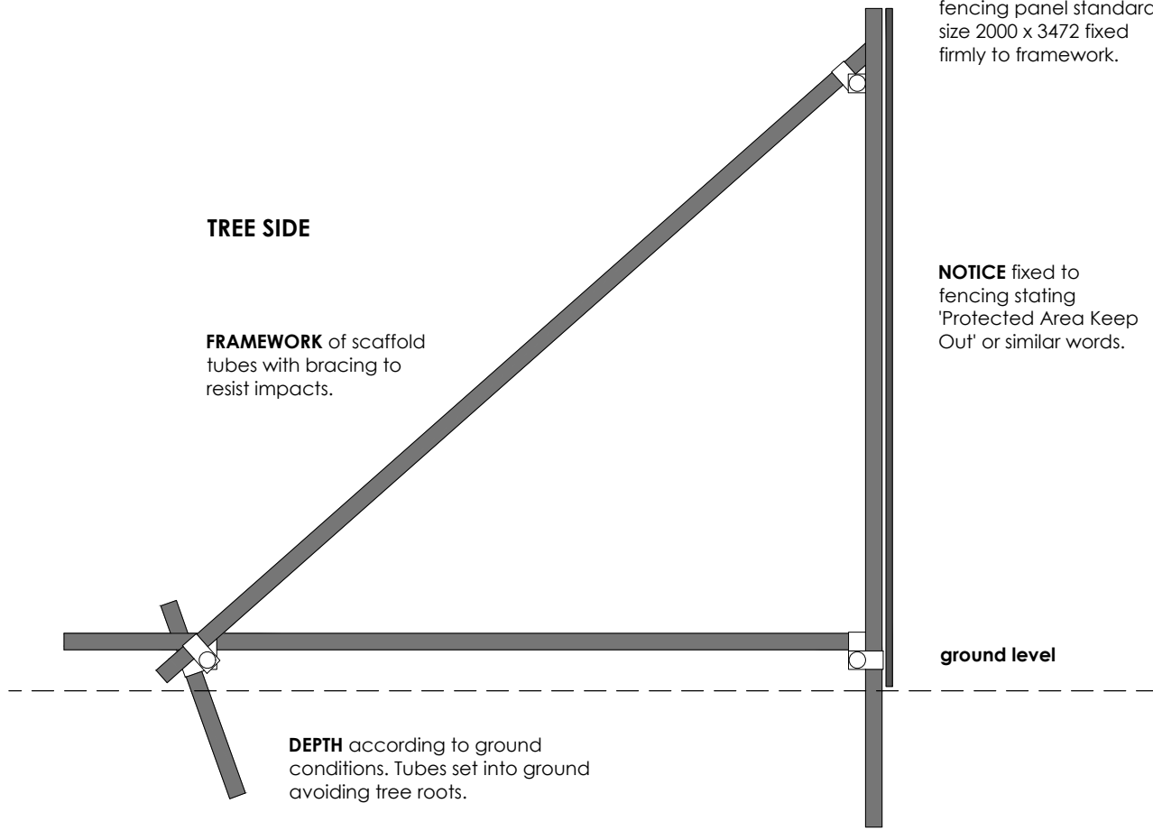
Tree Protection Fencing - Typical Detail 1:20
